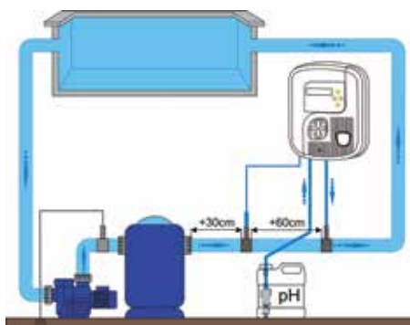
pH Expert installation diagram
